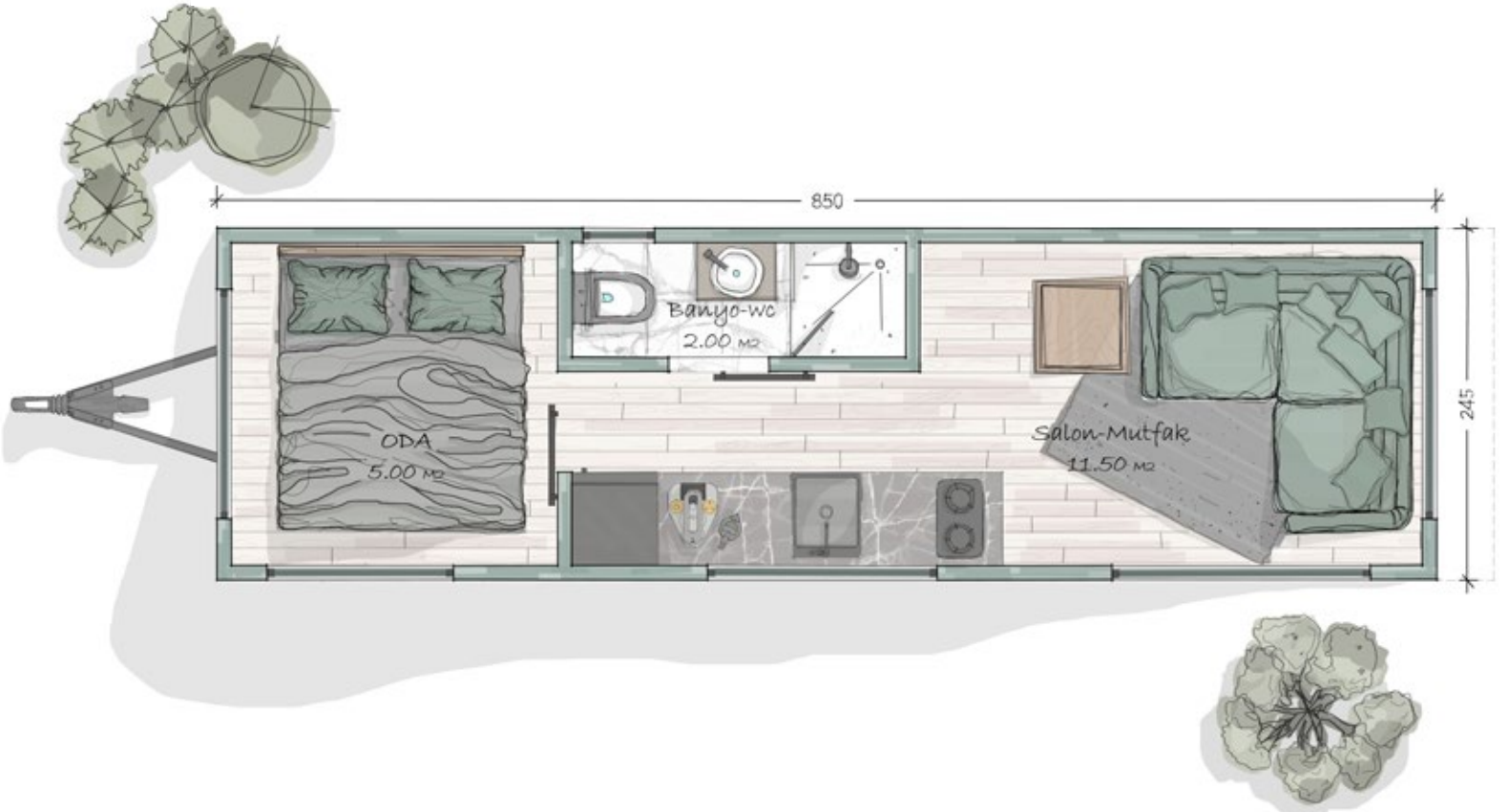
SUN-LIKYA PLANI-(20.5 m 2 )
